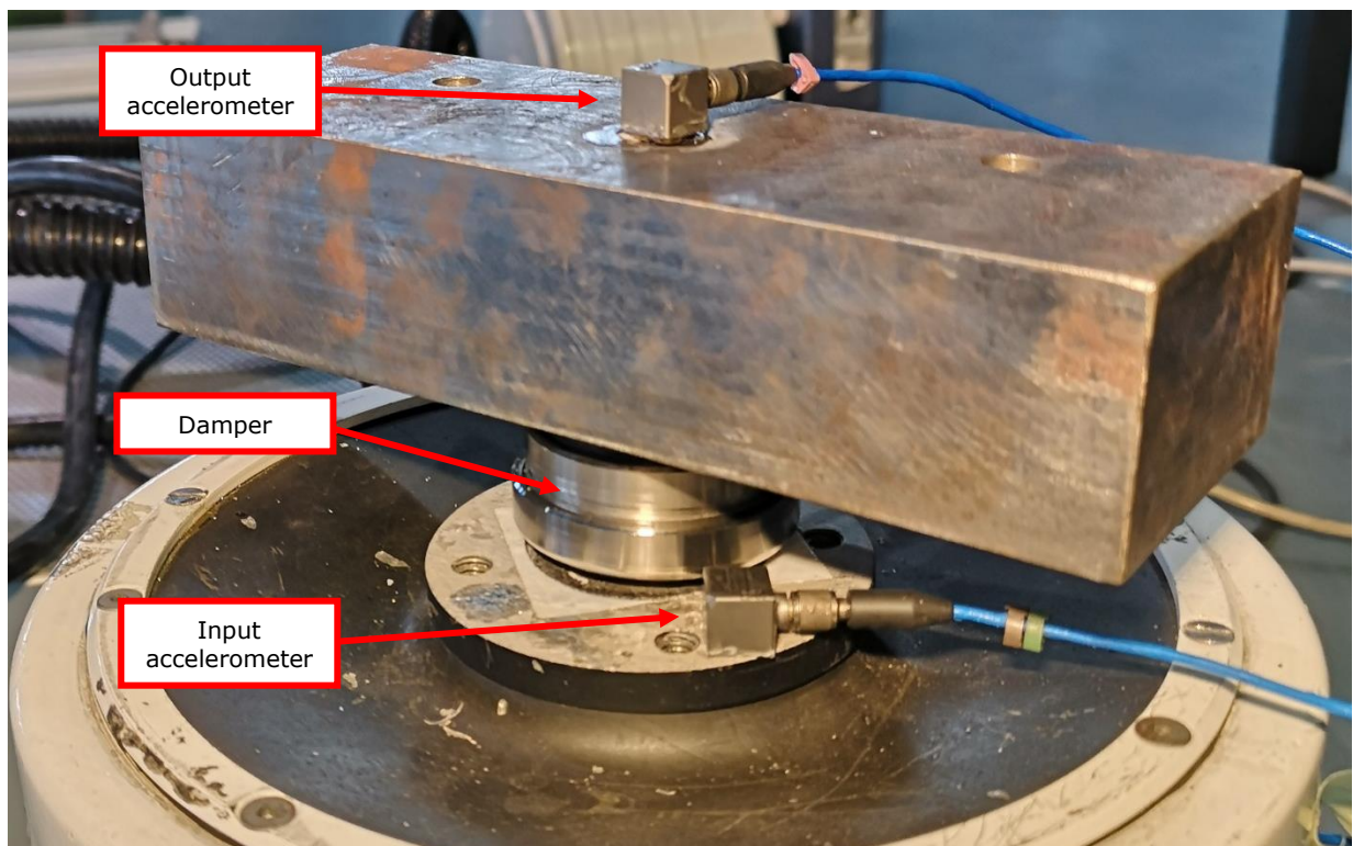
Figure 3. Test setup - Zoom.
