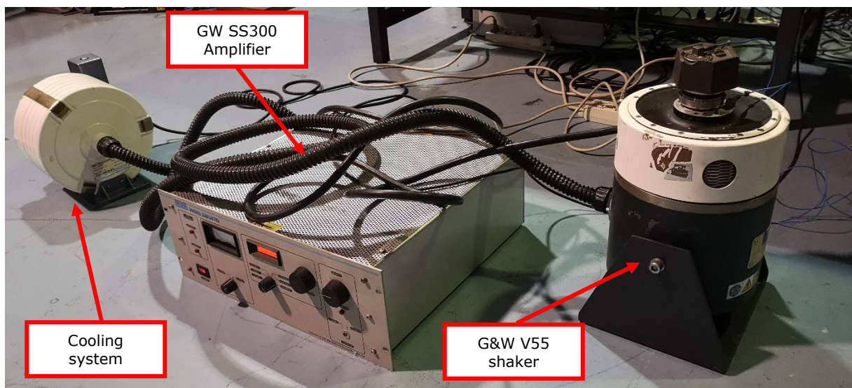
Figure 2. Testing systems.
