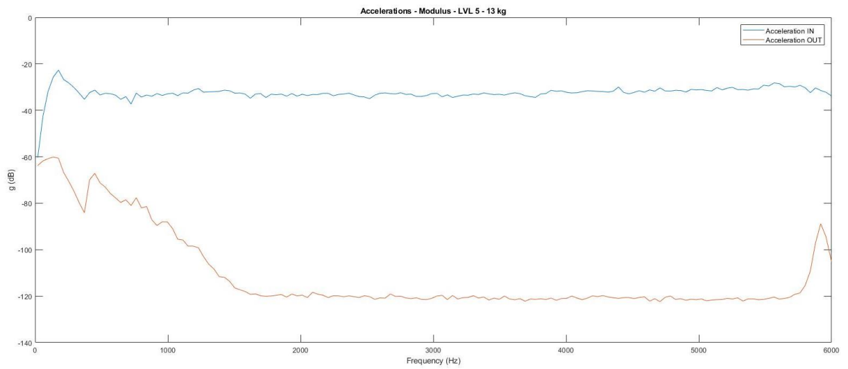
Figure 7. Incoming and outgoing accelerations on Level 5 damper loaded with 13 kg.
