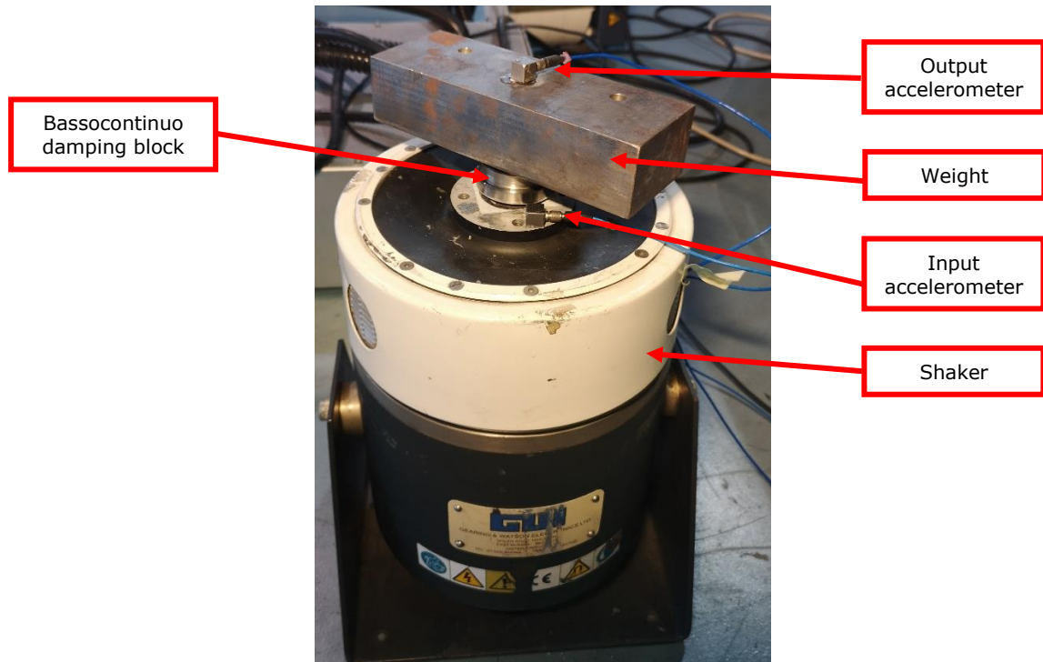
Figure 1. Test setup.
